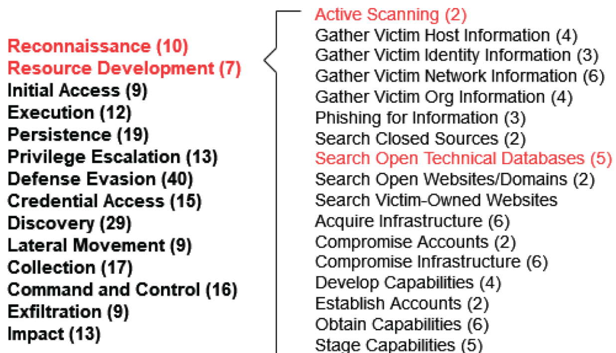
Figure 1.1 : MITRE Pre-ATT&CK
