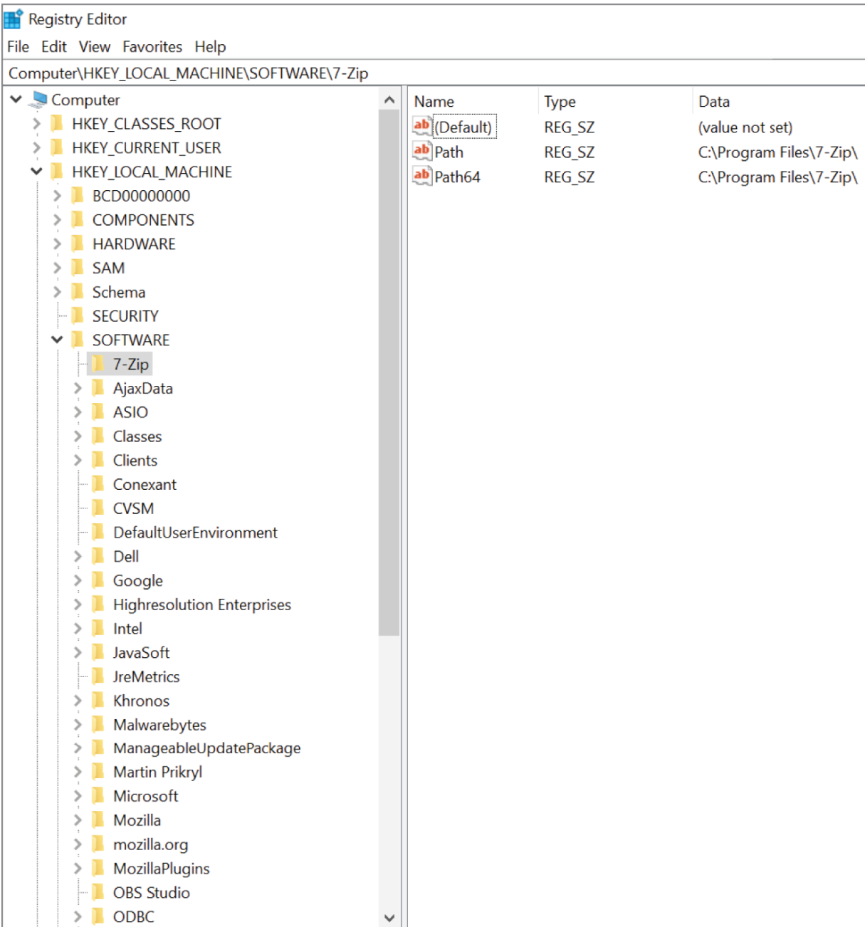
Figure 4.2: Windows Registry
