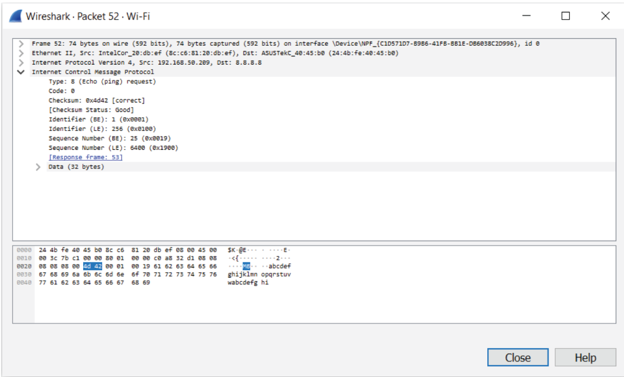
Figure 12.2: ICMP packet
